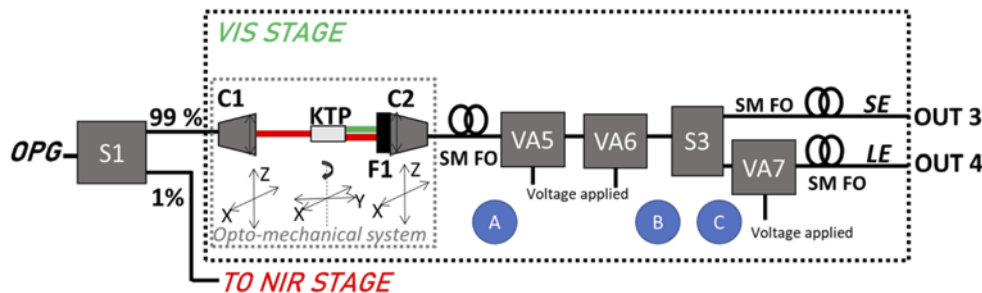
Fig. 7. Block diagram of VIS stage.
