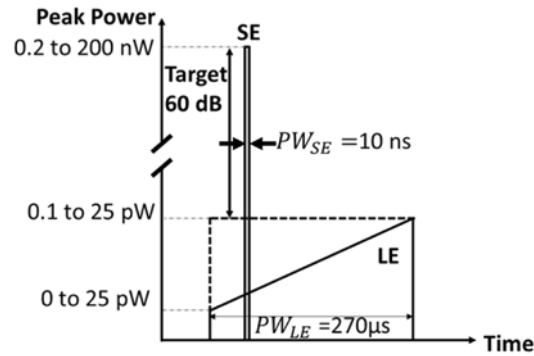
Fig. 1. Requirements for short (SE) and long echo (LE). Pulse width of the short echo. ( PW_{SE} ) and pulse width of the long echo ( PW_{LE} ).
