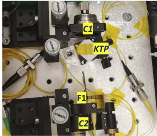
Fig. 8. The SHG setup in the VIS module.
