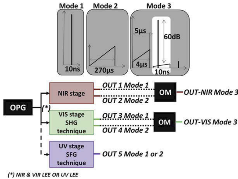
Fig. 5. Scheme of overall system design.
