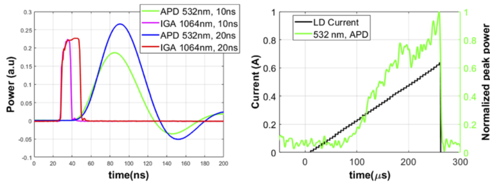
Fig. 14. The short echo (left) and ramp echo (right) measured by APD detector in VIS stage.
