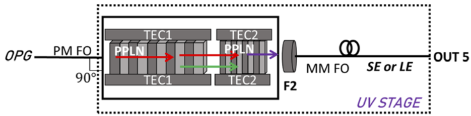
Fig. 9. Block diagram of UV stage.
