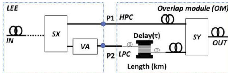
Fig. 4. Set-up for the technique of short and long echo overlapping.
