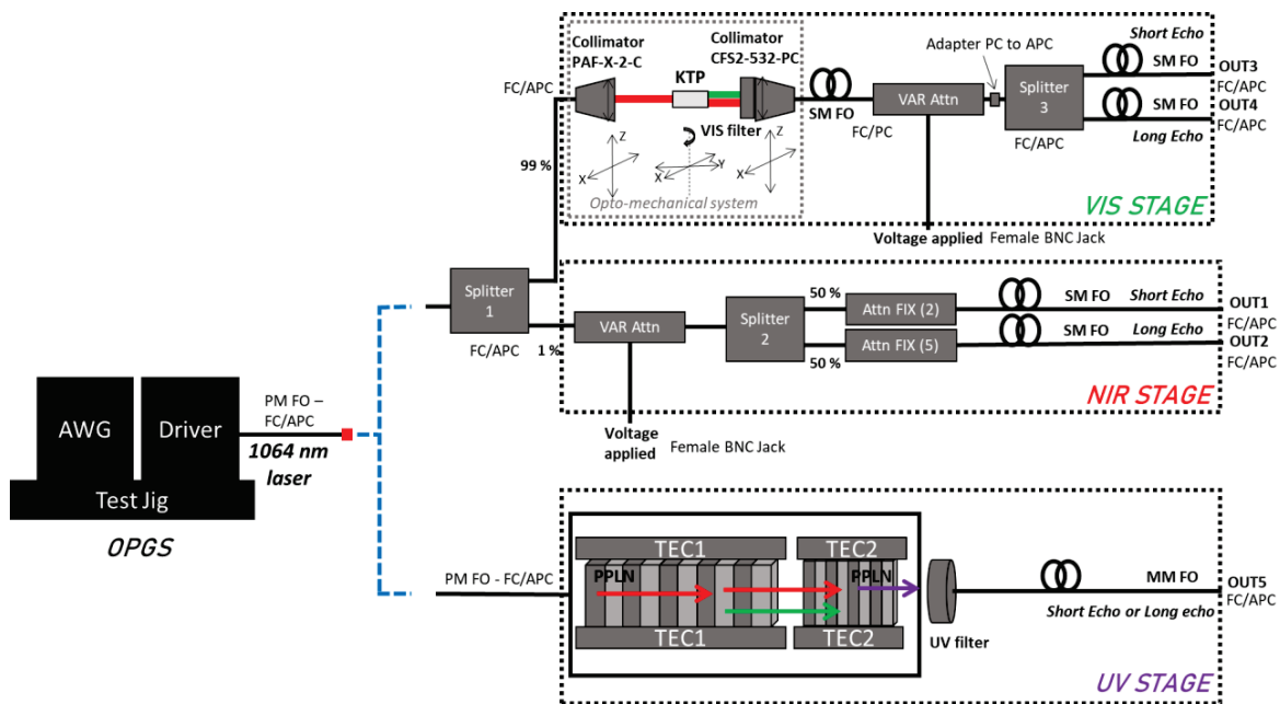
Figure 2. Block diagram of the complete system.
