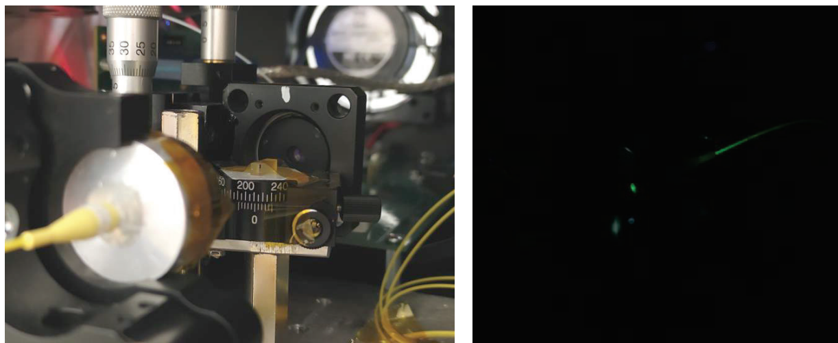
Figure 4. Set-up of SHG (left) and the beam at 532 nm passing through the VIS collimator (right).
