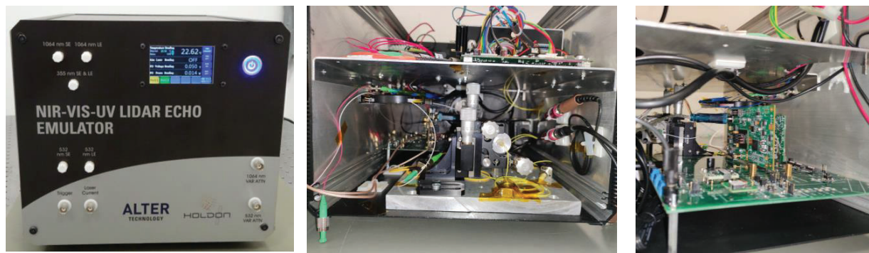
Figure 7. The front panel of NIR-VIS-UV LEE (left) and on the bottom level inside the LEE (center and right).
