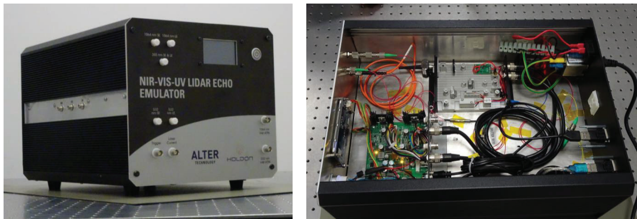
Figure 6. The transport unit of NIR-VIS-UV LEE (left) and on the top level inside the LEE (right).
