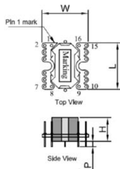
RM (Rectangular Module) based design with pins
